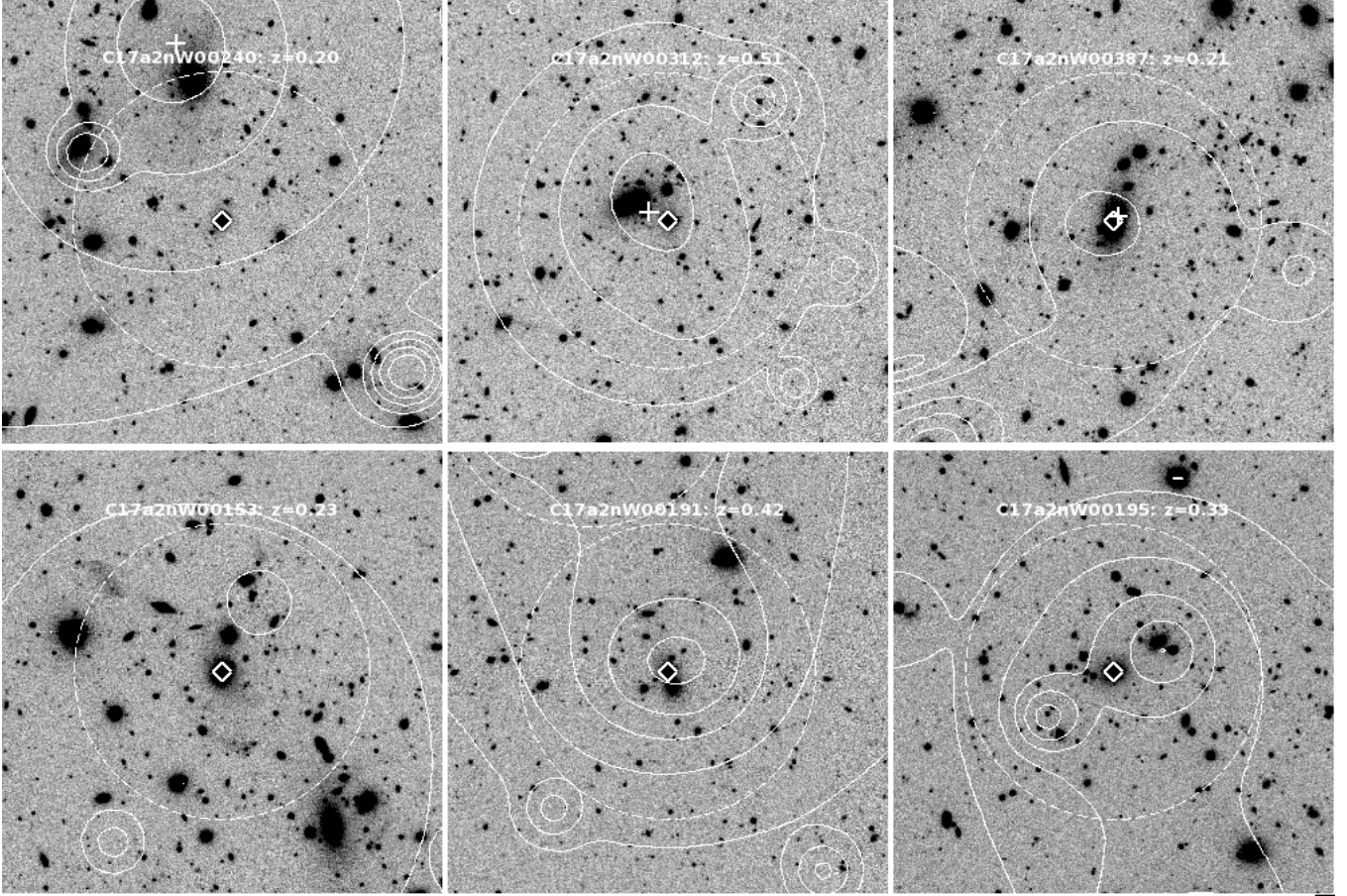
Figure 5. HSC i -band images of examples of clusters drawn from each sub-sample. Each image is three arcminutes on a side with north up and east left. XMM emission contours are shown in white. The XMM data in these images are processed using version 4 of the XamIn pipeline that combines individual pointings in to a mosaic. The dashed circle in each panel has a radius of 1 arcminute and is centered on the cluster location. The centroid of each CAMIRA detection is marked with a white diamond symbol. The centroid of each XXL detection is marked with a white cross symbol. Top panel: CAMIRA \log f_X > -14.2 (cgs) matched. Bottom panel: CAMIRA \log f_X < -14.2 (cgs) unmatched.
