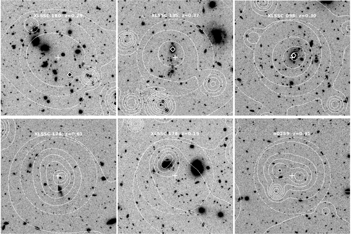
Figure 6. HSC i -band images of examples of clusters drawn from each sub-sample. Each image is three arcminutes on a side with north up and east left. XMM emission contours are shown in white. The XMM data in these images are processed using version 4 of the XamIn pipeline that combines individual pointings in to a mosaic. The dashed circle in each panel has a radius of 1 arcminute and is centered on the cluster location. The centroid of each CAMIRA detection is marked with a white diamond symbol. The centroid of each XXL detection is marked with a white cross symbol. Top panel: XXL N \geq 15 matched. Bottom panel: XXL N < 15 .
