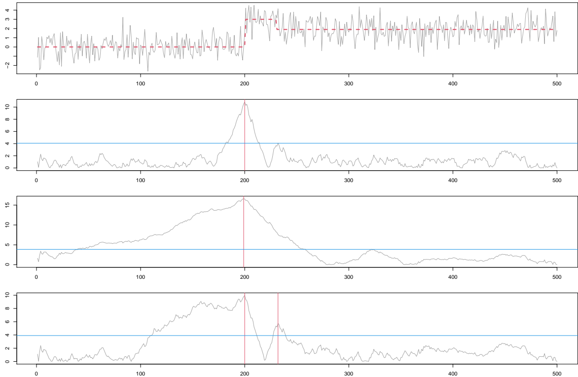
Figure 6: From top to bottom: A time series of length n = 500 with two mean changes at the locations 200 and 230 of respective height 3 and -1.1 , and the corresponding absolute MOSUM detector |T_{\mathbf{G}}(k)| for k = 1, \dots, n with (symmetric) bandwidths G = 30, 120 and \mathbf{G} = (30, 120) . Critical value at level \alpha = 0.05 is visualized by a solid horizontal line and the change-points estimated according to the \eta -rule by solid vertical lines.
