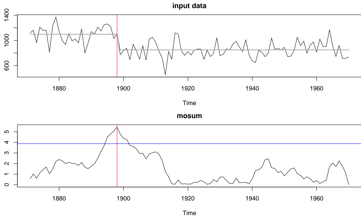
Figure 8: Annual flow of the Nile at Aswan from 1871 to 1970 with the estimated piecewise constant signal (above) and the corresponding values of the scaled absolute MOSUM detector with bandwidth G = 20 (below). The critical value is visualized by a solid horizontal line and the location of the estimated change-point location by a solid vertical line.
