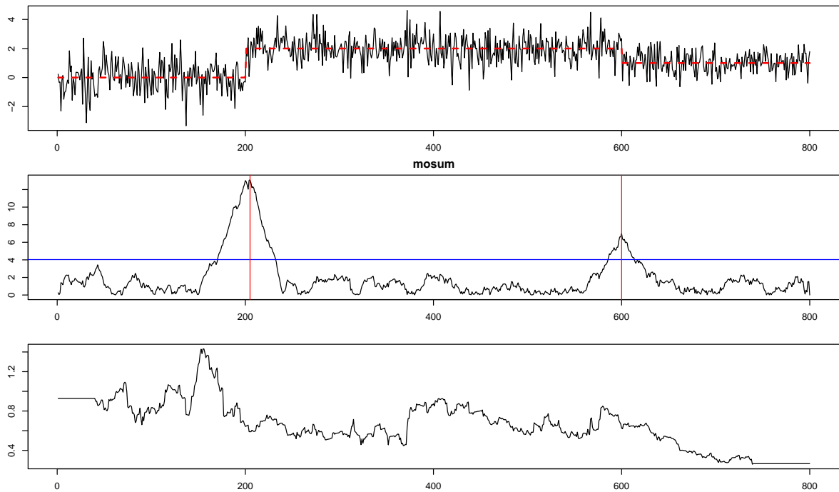
Figure 11: Top: A time series realization x_1 . Middle: The scaled absolute MOSUM detector. Bottom: Local variance estimator.
