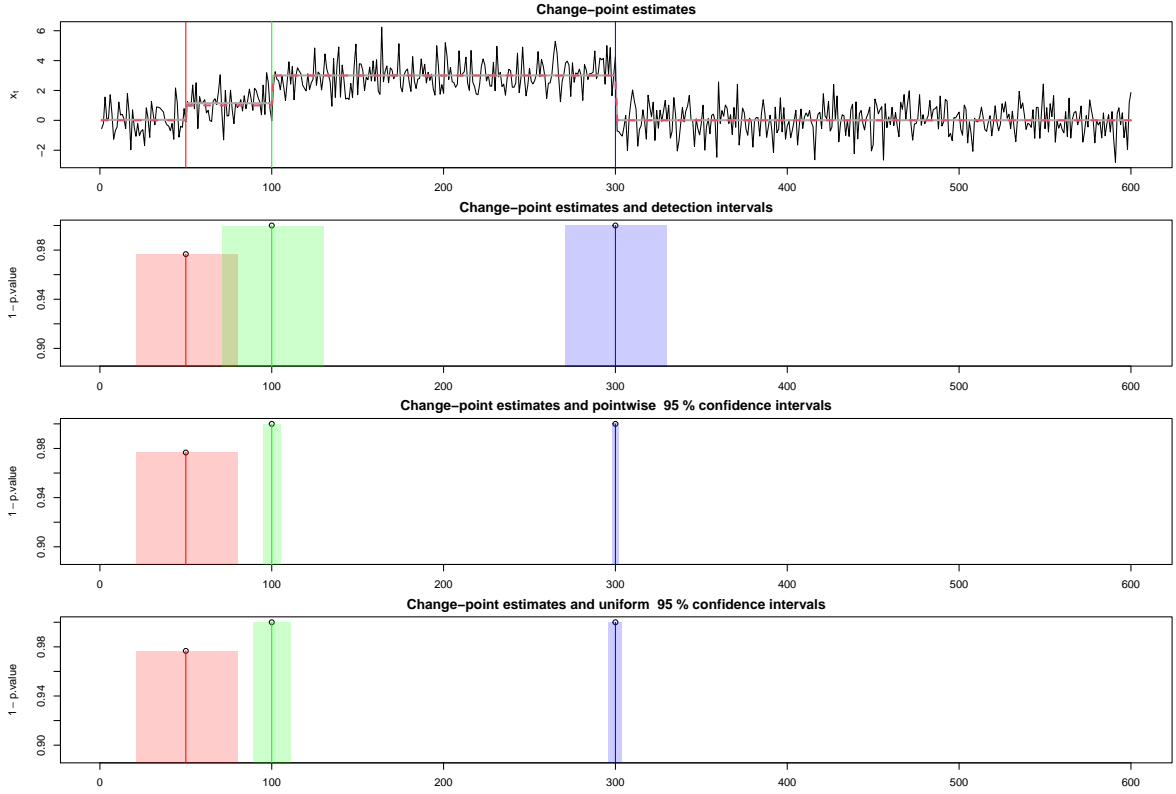
Figure 9: Top: A time series realization x , its underlying signal (dashed line), the change-point estimators (vertical lines) and the estimated piecewise constant signal (solid line). Below: Visualization of the significance of estimated change-points where the height of the vertical line at each estimated change-point location represents one minus the p values evaluated at the scaled absolute MOSUM detector value associated with its detection. The detection intervals of estimated change-points, the bootstrap pointwise confidence intervals K_j^{\text{pw}}(0.05) from (20) and the uniform confidence intervals K_j^{\text{unif}}(0.05) from (21) for j = 1, 2, 3 are visualized as shaded rectangles surrounding the vertical lines (second to fourth panels).
