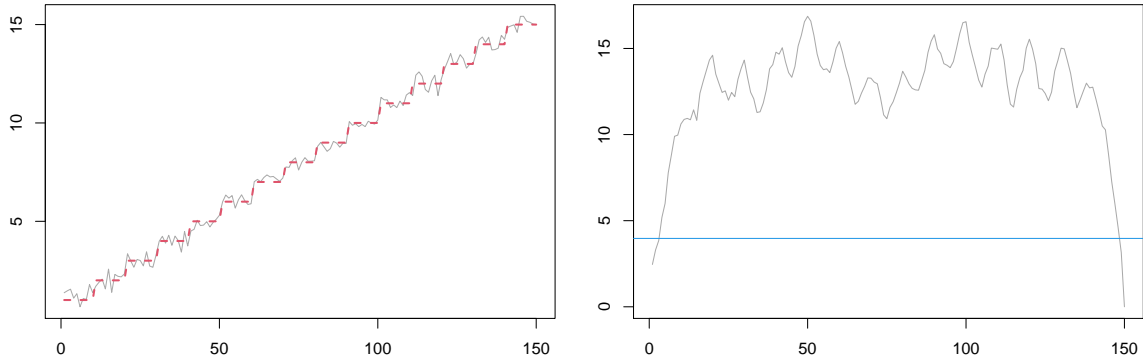
Figure 4: Left: A time series of length 150 with mean changes at locations 10, 20, \dots , 140, where the underlying step signal f_t is overlaid as dashed line. Right: The corresponding scaled absolute MOSUM detector \sigma^{-1}|T_G(k)| with G = 15 ; the critical value for level \alpha = 0.05 is denoted by a horizontal line. The series is a realization of the model stairs10 from Fryzlewicz (2014) (see Section 3.1).
