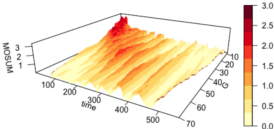
Figure 10: Surface plot visualization of the MOSUM detectors computed with a range of bandwidths on a realization of the mix test signal from Section 3.1.
