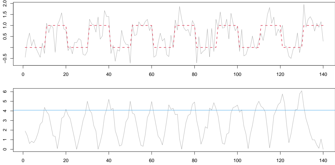
Figure 3: Top: A time series of length 140 with mean changes at locations 10, 20, \dots , 130, where the underlying step signal f_t is overlaid as dashed line. Bottom: The corresponding scaled absolute MOSUM detector \sigma^{-1}|T_G(k)| with G = 8 ; the critical value for level \alpha = 0.05 is denoted by a horizontal line. The series is a realization of the model teeth10 from Fryzlewicz (2014) (see Section 3.1).
