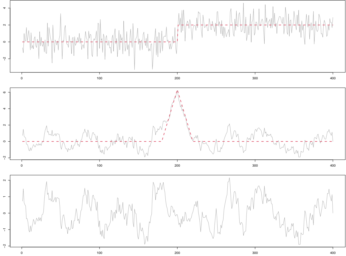
Figure 1: Top: A time series X_1, \dots, X_n of length n = 400 with one mean change of height d = 2 at time k = 200 . The corresponding step signal f_t is overlaid as dashed line. Middle: The MOSUM detector T_G(k; X) for k = 1, \dots, n , where the MOSUM signal T_G(k; f) is overlaid as dashed line. Bottom: T_G(k; e) = T_G(k; X) - T_G(k; f) .
