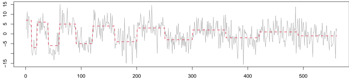
Figure 7: A realization from the mix time series model from Fryzlewicz (2014), with the piecewise constant signal overlaid in dashed line.
