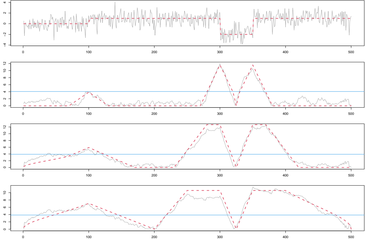
Figure 5: From top to bottom: A time series with mean changes at locations k_1 = 100 , k_2 = 300 and k_3 = 350 , where the underlying step signal f_t is overlaid as dashed line, and the absolute MOSUM detector |T_G(k)| for G = 30, 70 and 100 , where the absolute MOSUM signal |T_G(k; f)| is overlaid as dashed line and the critical value at level \alpha = 0.05 is visualized by a solid horizontal line.
