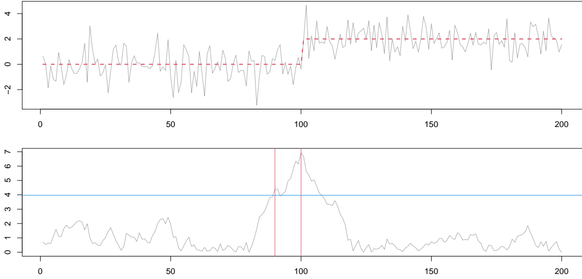
Figure 2: Top: A time series with one mean changes at the location 100, where the underlying step signal f_t is overlaid as dashed line. Bottom: The corresponding absolute MOSUM detector |T_G(k)| for k = 1, \dots, n with bandwidth G = 20 . The critical value for level \alpha = 0.05 is denoted by a horizontal line, and maximal points within significant environments of T_G(k) are highlighted by the vertical lines.
