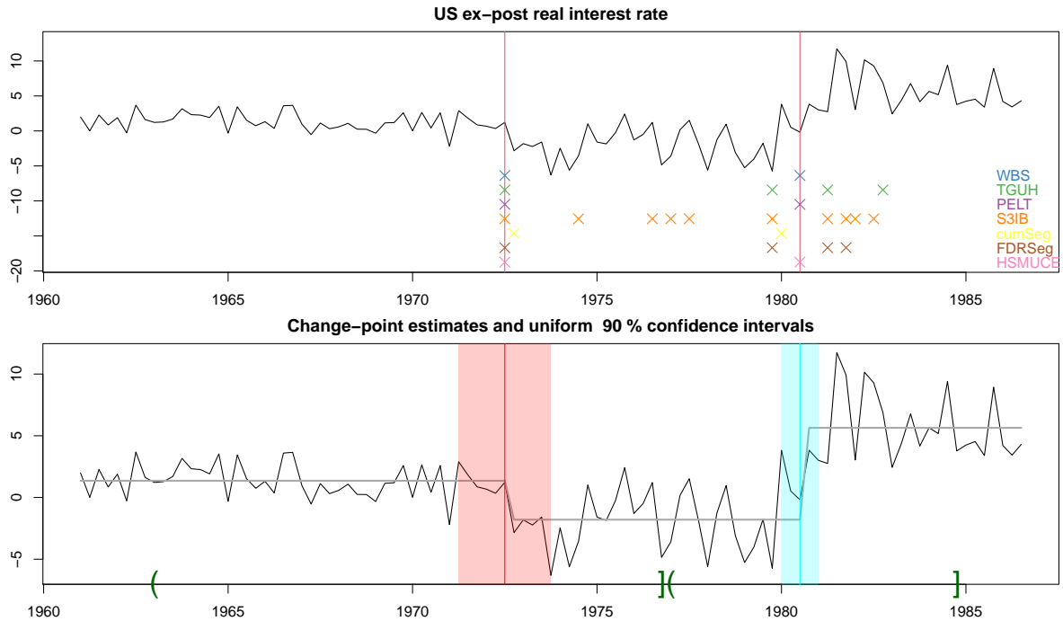
Figure 12: Top: The quarterly US ex-post real interest rate from 1961:Q1 to 1986:Q3, where the vertical lines denote the two change-point estimators returned by multiscale.localPrune . Also plotted are change-points estimated by the WBS, TGUH, PELT, S3IB, cumSeg, FDRSeg and H-SMUCE. Bottom: The 90% confidence intervals of change-point locations produced by confint (shaded areas) and the function jumpoint of stepR (plotted on the x -axis) against the input time series and the estimated piecewise constant signal.
