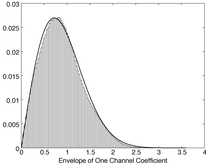
Fig. 2. Histogram of the envelope of one channel coefficient for an NLoS indoor MIMO scenario and a Rayleigh pdf (normalized).
