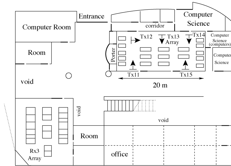
Fig. 1. Measurement scenario for the NLoS indoor MIMO channels.
