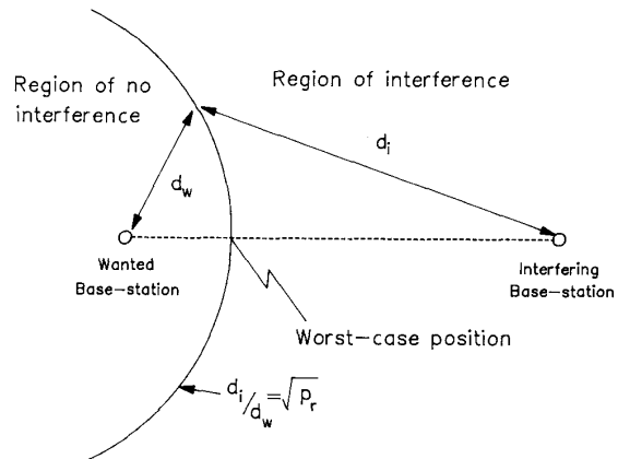
Fig. 4. Contour defining interference regions.
