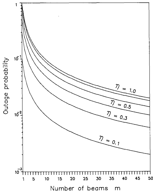
Fig. 5. Outage as a function of the number of beams.
