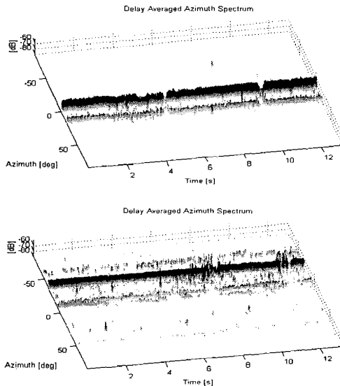
Fig. 4. Variation in multipath angle of arrival (estimated at the AP for one MT antenna element) for (top) Location A, (bottom) Location B. Both plots have had a threshold applied at -40\text{dB} from their peak components.
