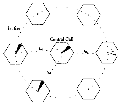
Figure 1: Cellular layout (Up and Down links).
