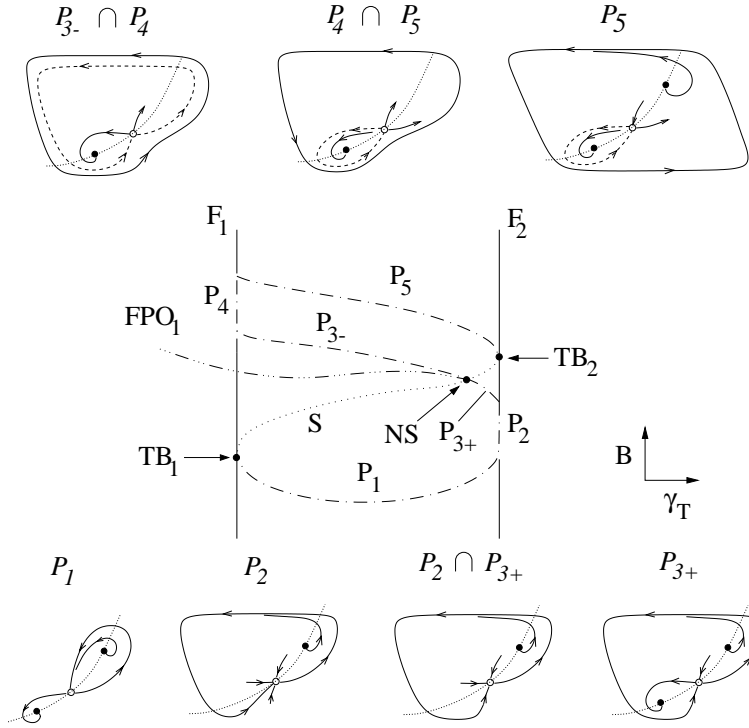
Figure 11: The qualitative depiction of the homoclinic bifurcation scenario.
