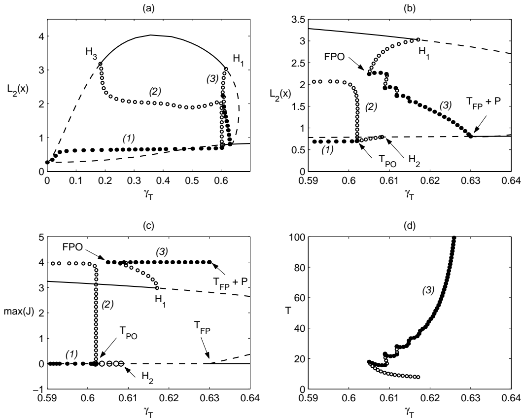
Figure 13: One-parameter bifurcation diagram at B = 0.8055 ( u = 40 ). (a) L_2 norm vs. parameter. (b) A zoom showing the birth and death of the classic surge cycle (branch (3)). (c) \max(J) vs. \gamma_T . Note that although the L_2 norm of branch (3) tends to the fixed point in panel (b), the maximum of the J component remains large. Thus, along a classic surge cycle, rotating stall fully develops and dies away. (d) Period T vs. parameter, showing the homoclinic nature of the classic surge cycle.
