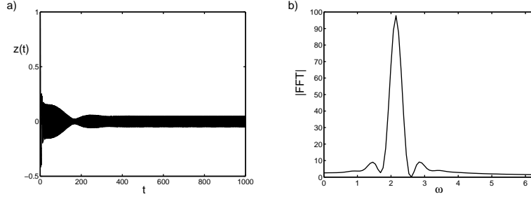
Figure 7. (a) Solution z(t) with \tau = 1.55 , k = 0.01 , \Omega = 2.1 , p = 0.75166 . (b) Fourier spectrum of the solution.
