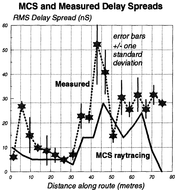
ENGINEERING SCHOOL Indoor Corridor Route FIGURE 5
