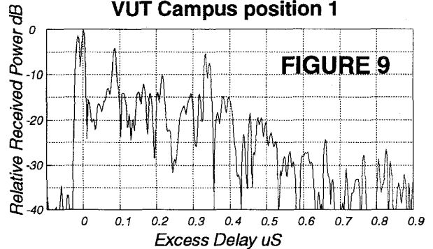
Power Delay Profile rms delay spread 126nS VUT Campus position 1
