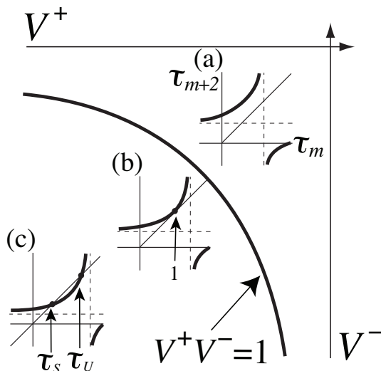
FIG. 4.1. Tangent mapping and bifurcation diagram: (a) no invariant manifolds for V^+V^- < 1 , (b) bifurcation along V^+V^- = 1 , (c) two fixed points \tau_S = \tau_* and \tau_U = 1/(\tau_*V^+V^-) in V^+V^- > 1 . \tau_m = 0 is the boundary of \Sigma^{\text{esc}} . Lines with \tau_m = 2 - 1/(2V^+V^-) map to the \tau_{m+2} graph asymptotes (dashed) which are the boundaries of \Sigma^{\text{sl}} . The bound \tau_m < 2 ensures the existence of the intermediate step \tau_{m+1} .
