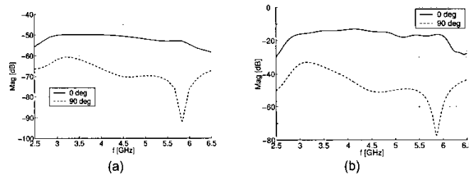
Fig.6 Transfer Functions: (a) H_{rx}(f) -Rx mode, (b) H(f) -2-antenna system.
