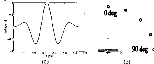
Fig.2 (a) Excitation pulse, (b) time-domain probes.
