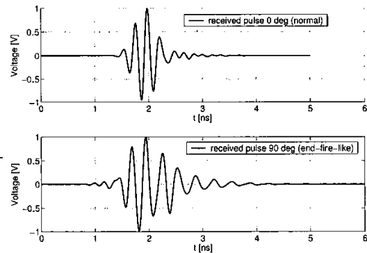
Fig.8 Received pulses.
