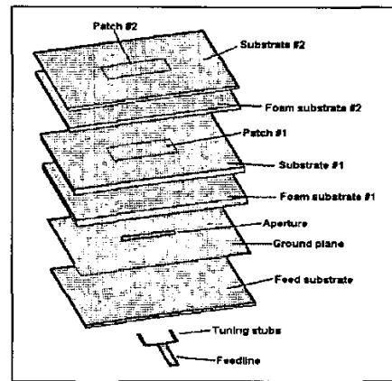
Fig.3 The geometry of ASPA.
