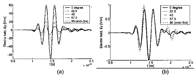
Fig.7 Radiated pulses: (a) absolute values, (b) normalized values.
