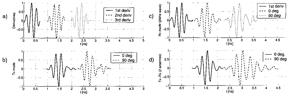
Fig.9 Comparison between ideal derivative of input signals and output waveforms (0 and 90 deg propagation directions): a) input pulse derivatives, b) Tx mode, c) Rx mode, d) for 2-antenna system.
