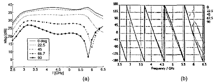
Fig.5 H_x(f) : a) amplitude [dBV/m], b) phase [degrees].
