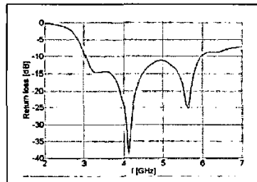
Fig.4 Return loss of ASPA.
