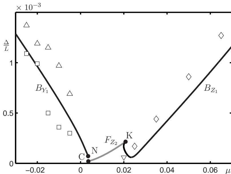
Figure 3: Partial bifurcation diagram of Equations (15) in the (\mu, \Delta/L) -plane showing a curve F_{Z_2} of fold bifurcations of Z_2 and curves B_{Z_1} and B_{Y_1} of branch points of Z_1 and Y_1 , respectively. Also shown are experimental data points; here \square indicates the largest \Delta/L -value where only Z_2 was detected, \triangle where Y_1 was detected for the first time, \diamond where Z_1 was detected for the first time, \nabla that Y_2 was detected.
