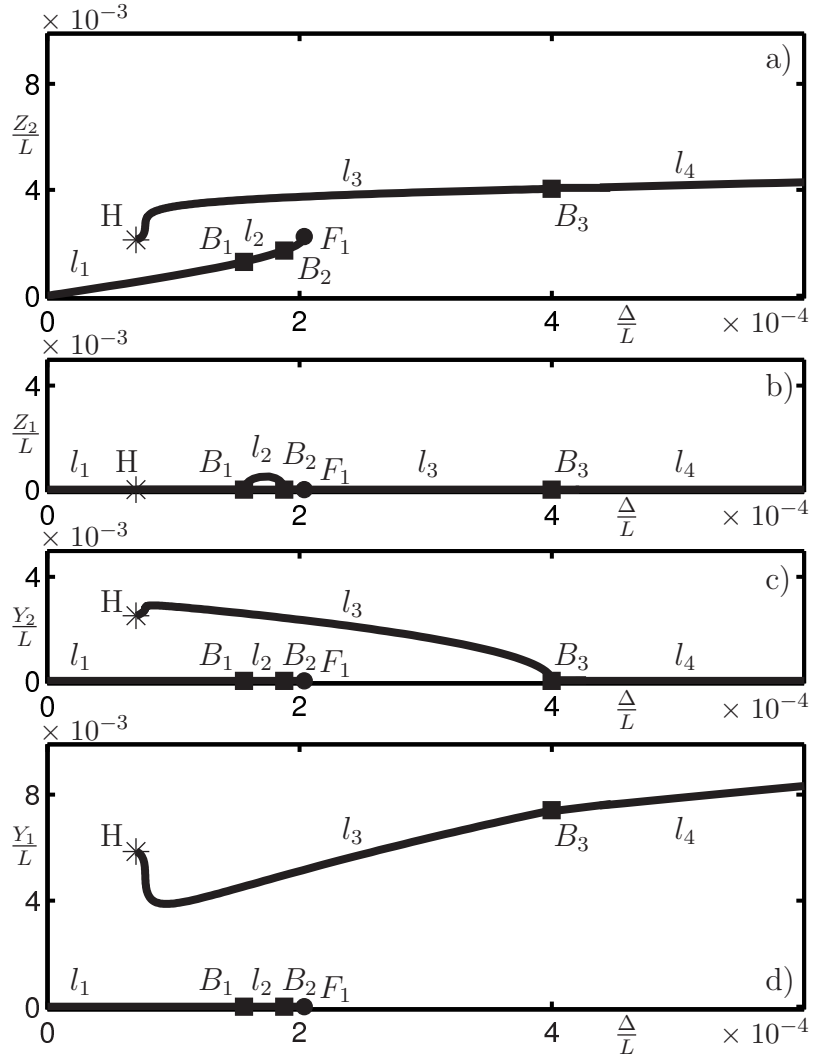
Figure 6: Mode contributions to the stable branches l_1 - l_4 from Figure 5 ( \mu = 0.02 ), showing the contribution of a) Z_2 , b) Z_1 , c) Y_2 , and d) Y_1 .
