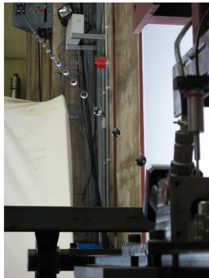
Figure 2: Apparatus for inclined cable experiment: a) side view, b) looking along cable from bottom, c) hydraulic actuator and load cell. The cable is 5.4 m long, has diameter 0.00078 m and is inclined at 22.6^\circ . The lead masses are applied to increase the cable mass for more realistic scaling. Deck excitation is simulated with the hydraulic actuator positioned at the lower attachment point.
