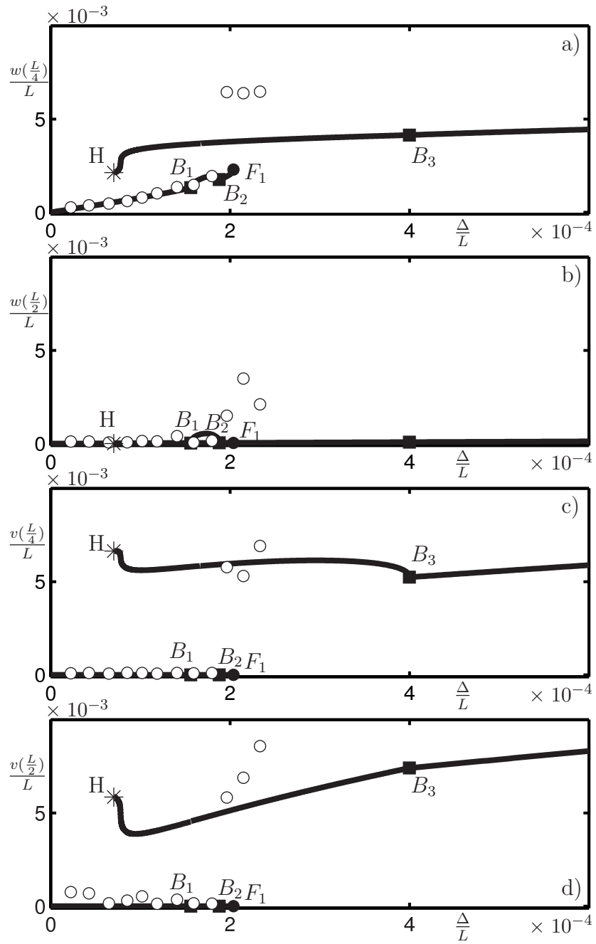
Figure 7: Comparison of theoretical maximum displacement with experimental measurements for \mu = 0.02 . Shown are measured data points of displacement (denoted by \circ ), together with theoretical values along the stable branches l_1 - l_4 of a) W(\frac{L}{4})/L , b) W(\frac{L}{2})/L , c) V(\frac{L}{4})/L , and d) V(\frac{L}{2})/L .
