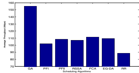
Figure 5: Average Throughput for different scheduling algorithms with joint time-frequency scheduling
