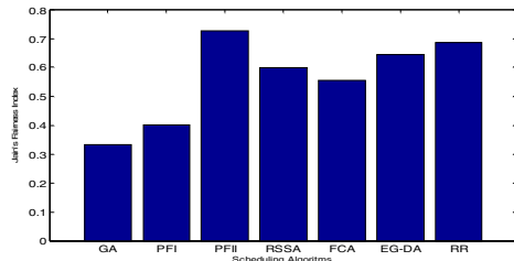
Figure 6: Jain's Rate Fairness Index for different scheduling algorithms with joint time-frequency scheduling
