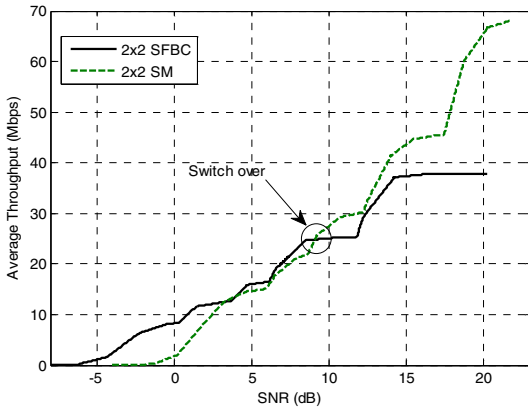
Figure 2: Switching point for SFBC and SM schemes
