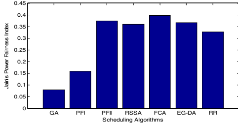
Figure 7: Jain's Power Fairness Index for different scheduling algorithms with joint time-frequency scheduling
