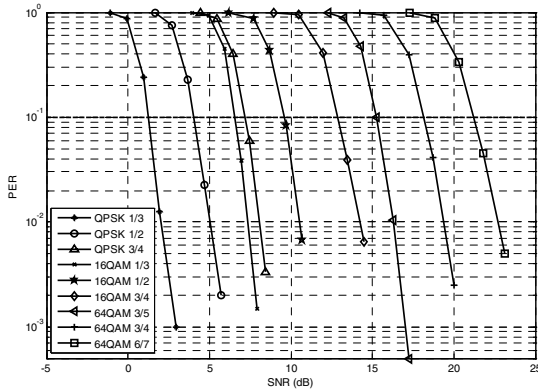
Figure 1: PER vs SNR for different MCSs
