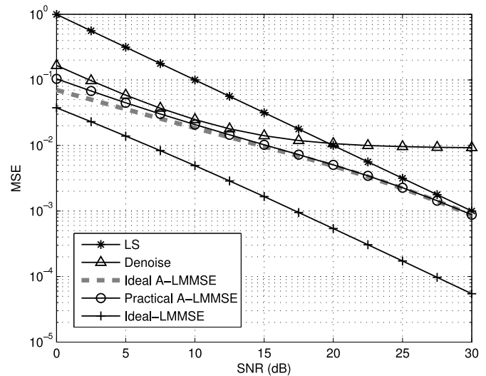
Fig. 8. MSE comparison of DFT-based channel estimators
