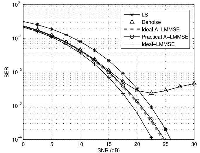
Fig. 9. BER of LFDMA with different DFT-based channel estimators
