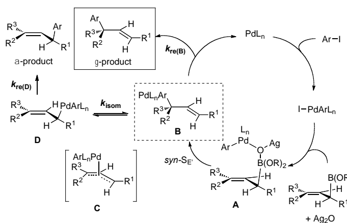
Scheme 1. Mechanism for the formation of both the \alpha - and \gamma -isomers
