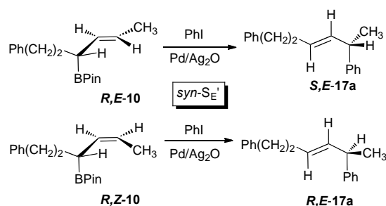
Scheme 2. Absolute configuration of products and the relationship to mechanism of transmetalation
