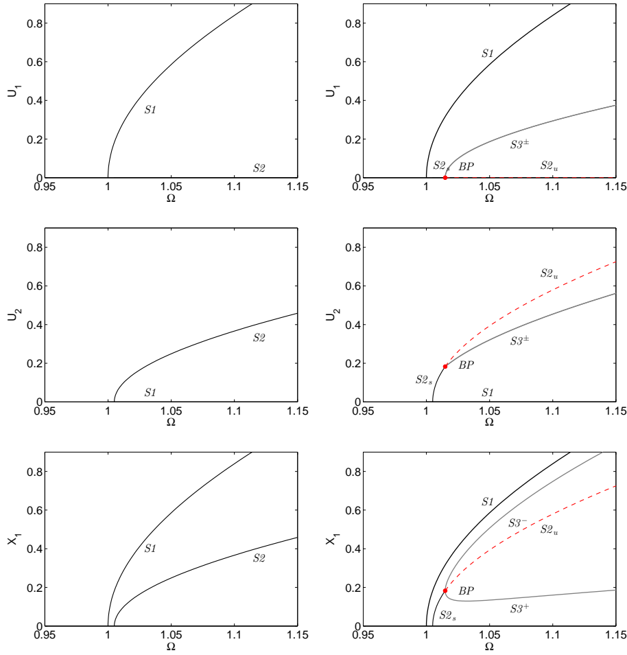
Fig. 2: Backbone curves for \omega_{n1} = 1 , \omega_{n2} = 1.005 , \kappa = 0.4 . The panels in the first and the second column show the cases \kappa_2 = 0.2 ( \kappa < 4\kappa_2 ) and \kappa_2 = 0.05 ( \kappa > 4\kappa_2 ) respectively. In the first and second row, the projection of amplitude of the fundamental response in terms of u_1 and u_2 is shown. In the third row, the backbone curves are represented in the projection of amplitude of displacement of the first mass. Stable solutions are shown with solid black lines, whereas unstable solutions are represented by dashed red lines. Bifurcation points are indicated with red bullets labelled BP. (Strictly these are the secondary bifurcations points as defined by Lewandowski [?,?]).
