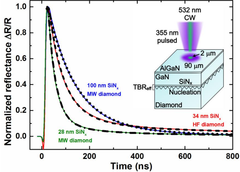
FIG. 1. Normalized transient thermoreflectance measured on three GaN-on-diamond wafers with 100 nm, 34 nm and 28 nm-thick SiN x layers on either the opaque hot filament (HF) CVD diamond or the translucent microwave (MW) plasma CVD diamond. Best fit curves are overlaid with results given in TABLE I. Inset shows a schematic of the measurement.
