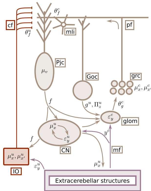
Figure 7. Olivo-cerebellar circuitry. Mapping of elements of the model for a conditioning paradigm to elements of the olivo-cerebellar circuitry. The mossy fibre pathway is the same as in Fig. 2, but here it is exclusively concerned with the estimation of the conditioned stimulus (c superscript). The inferior olive-climbing fiber pathway, instead, is concerned with the estimation of the unconditioned stimulus (u subscript), also based on a state space model (Eq. 23). In practice, the inferior olive (IO) could receive prediction errors \varepsilon_y^u about the unconditioned stimulus from extra-cerebellar structures, as shown in Fig. 1—illustrating message passing between neuronal structures. Meanwhile, the IO would also receive predictions f about the motion of unconditioned states, \mu_x^u , from CN-mediated PjC input. Together, error and prediction input would drive expectations encoded by IO neurons about the unconditioned stimulus, \mu_x^u, \mu_{x'}^u . Notably, the comparison between predicted, f , and expected motion of the unconditioned state, \mu_x^u , encoded by error units \varepsilon_x in the IO, would drive cf activity and subsequent updates of expectations about the control state, \mu_v , encoded in the PjC population. In a conditioned paradigm, the climbing fibre pathway described above is responsible for the estimation of the unconditioned stimulus that drives baseline behavioural response pattern in extra-cerebellar structures. Following learning, the presentation of the conditioned stimulus becomes associated with the unconditioned stimulus, and can elicit a response on its own, called conditioned response. Associative learning in the cerebellum involves changes in the pf connectivity matrix, \theta_f^c , and, similarly to inference, it complies with the free energy minimisation imperative, but on a slower time scale: thus, learning can be specified with a gradient descent on free energy with respect to \theta_f . In this specific case, for example, \theta_f^c would increase in value because the cerebellar model that best explains IO and mf input is the one which expects the control state \mu_v , indicating the behavioural context, to generate both unconditioned, \mu_x^u , and conditioned states, \mu_x^c .
