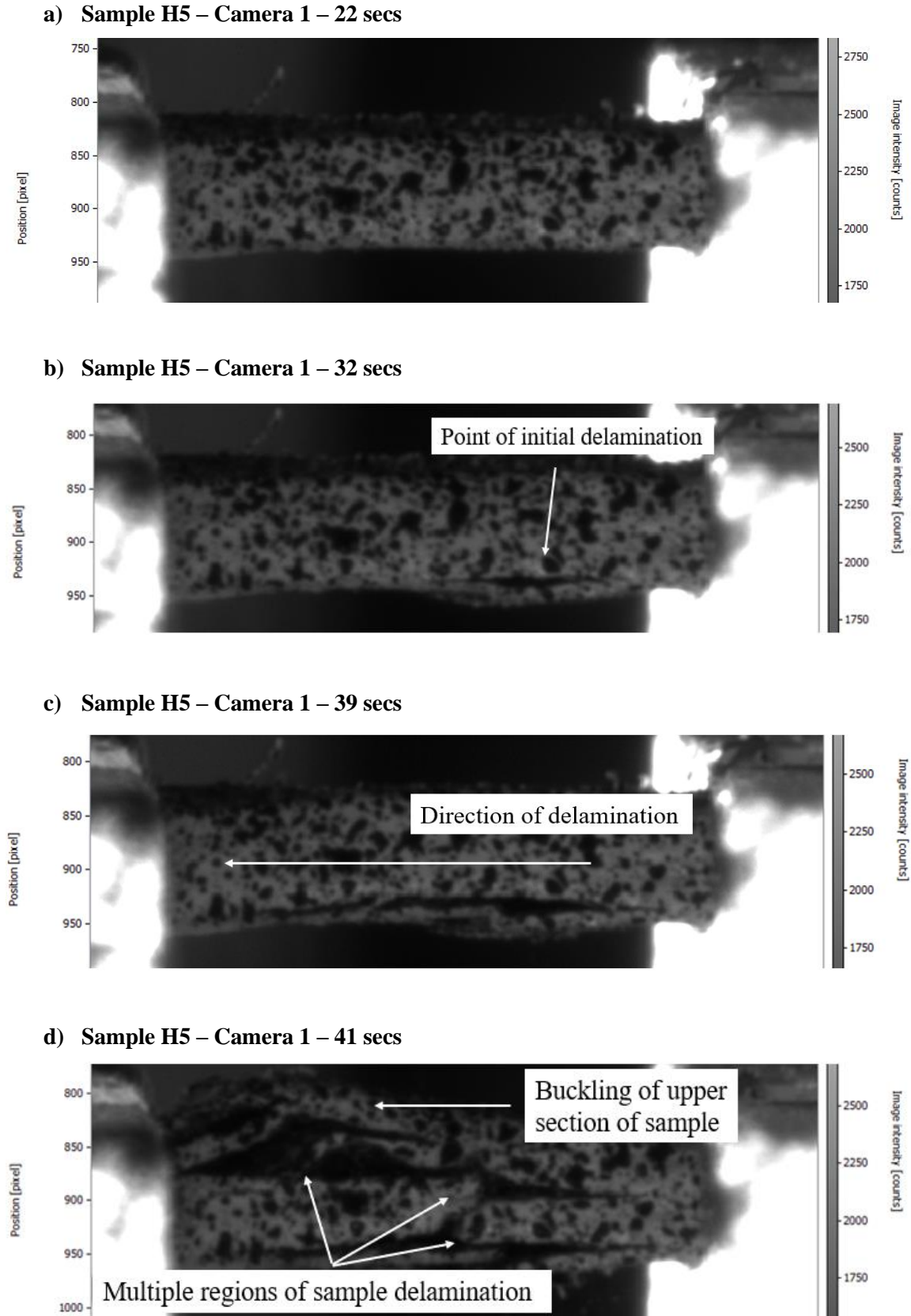
Figure 6: A timeline of failure for sample H5, illustrating progressive interlaminar delamination prior to an eventual buckling of the remaining material.
