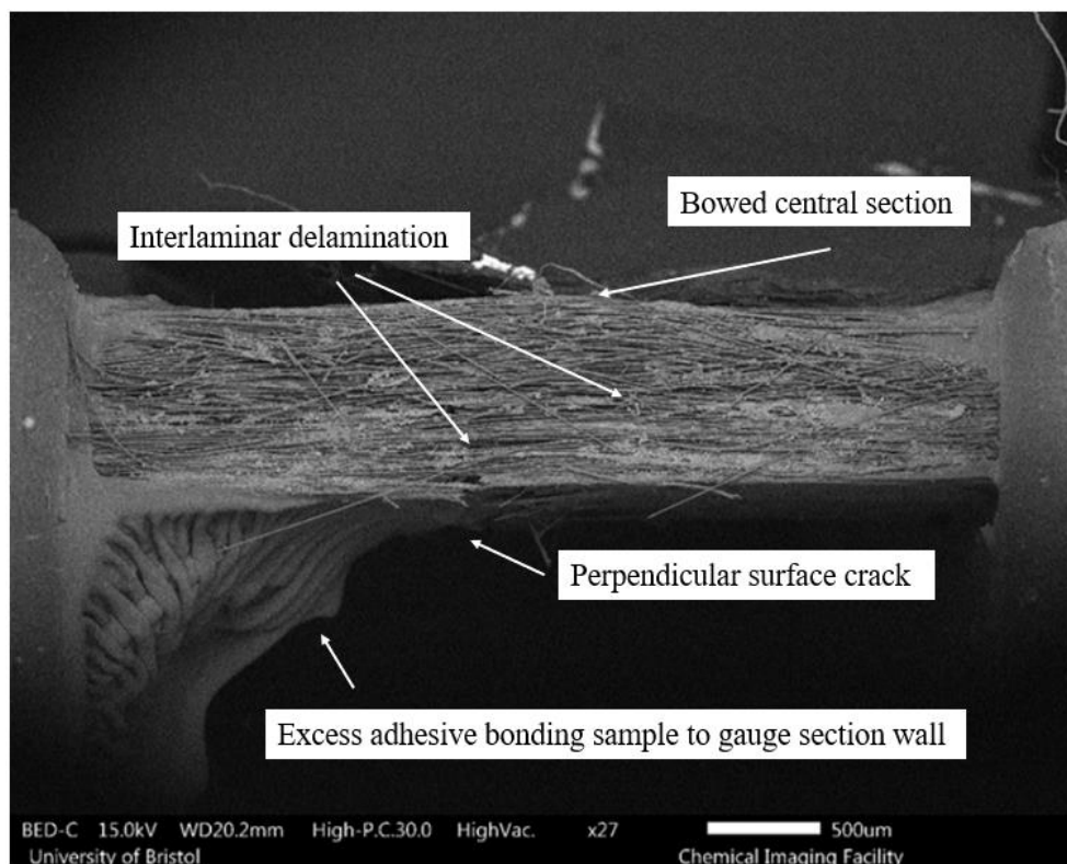
Figure 5: SEM micrograph of unpainted sample H16, scale bar length 500 μm.
