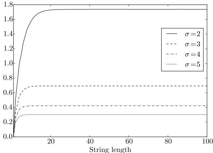
Fig. 1: Average difference between the length n of a string and the length of its maximal unbordered factor for 1 \leq n \leq 100 and alphabets of size 2 \leq \sigma \leq 5 .
