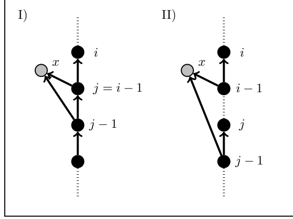
Figure 4: General food web configuration consisting of a chain of specialists and an omnivore x . In I) the omnivore x feeds on two subsequent trophic levels, i.e. i = j + 1 , whereas in II) the omnivore x feeds on two non-subsequent trophic levels, i.e. i > j + 1 . Accordingly, different coexistence ranges are obtained for both cases, as described in the text.
