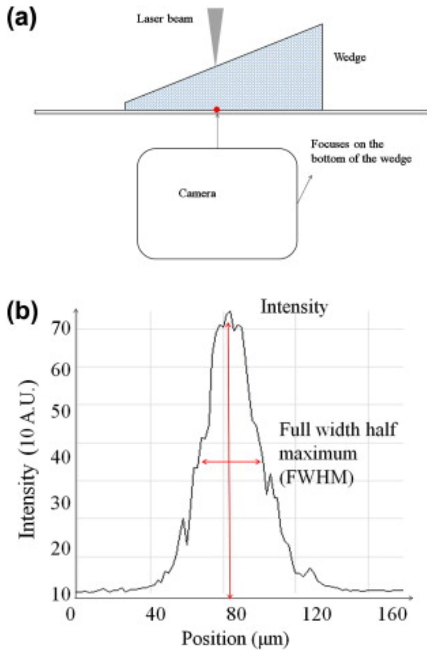
(a) Schematic of experimental set-up and (b) a typical laser intensity profile and the definition of the beam diameter.
