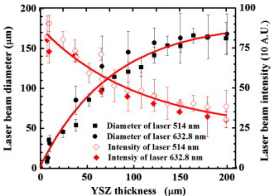
The variation of red ( \lambda = 632.8 \text{ nm} ) and green laser ( \lambda = 514 \text{ nm} ) beam diameters with APS-YSZ thickness.
