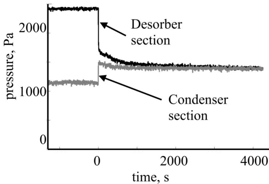
Figure 3 Pressures inside the two sections of the calorimetric apparatus. The connecting valve was opened at time = 0 s. (a) conditions for adsorption, evaporator temperature = 303K and adsorbent temperature = 306 K [1] (b) conditions for desorption, with adsorbent temperature = 303K and condenser temperature = 283 K. Part (a) reprinted from Applied Thermal Engineering , Vol. 40, M. A. Ahamat and M. J. Tierney, Calorimetric assessment of adsorbents bonded to metal surfaces , Copyright 2012, with permission from Elsevier.
