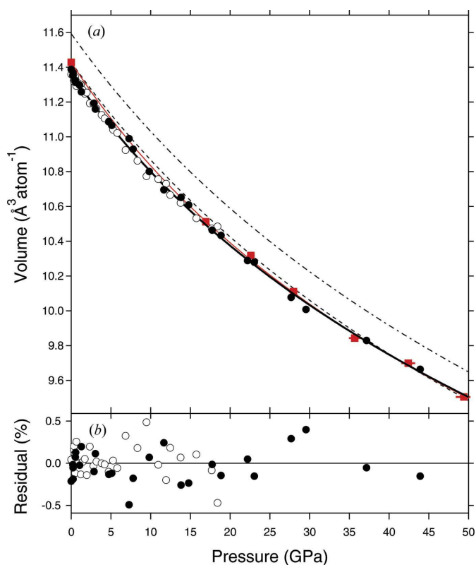
Figure 4 Volume per atom for B20- \text{Ni}_{53}\text{Si}_{47} as a function of pressure as calculated from the Cu pressure marker using the EoS of Dewaele et al. (2004; circles). The filled circles are from experiment 1 (in Ne) and the open circles from experiment 2 (in He). The thick solid line is a third-order Birch–Murnaghan EoS fitted to all the data (Table 2). The dashed line is the EoS fitted to the ab initio simulations from Vočadlo et al. (2012), which has been corrected so that its V_0 is equal to that of the experimentally determined value. The uncorrected ab initio EoS is represented by the dash-dot line. The thin solid red line is the EoS fitted to the P - V data of Lord et al. (2012; red squares), which was produced using NaCl as the pressure medium coupled with laser annealing on a stoichiometric NiSi sample.
