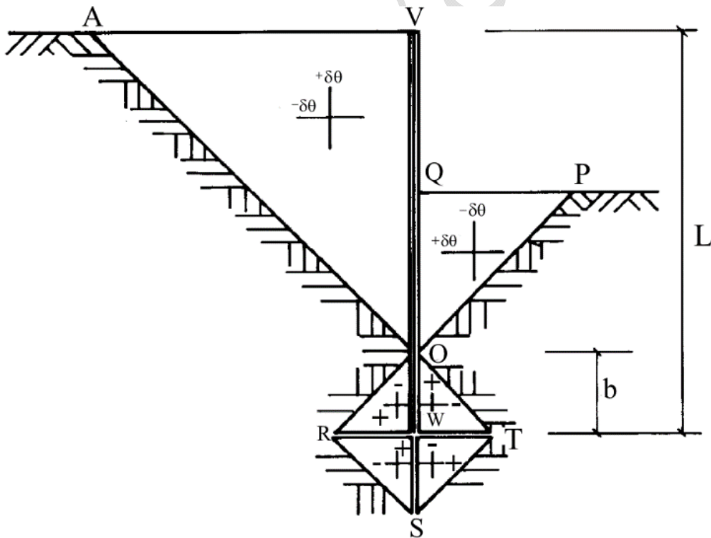
Figure 2: Admissible strain field for embedded cantilever wall rotating about a point just above its base: Rigid wall (adapted from Bolton and Powrie 1988, with permission
