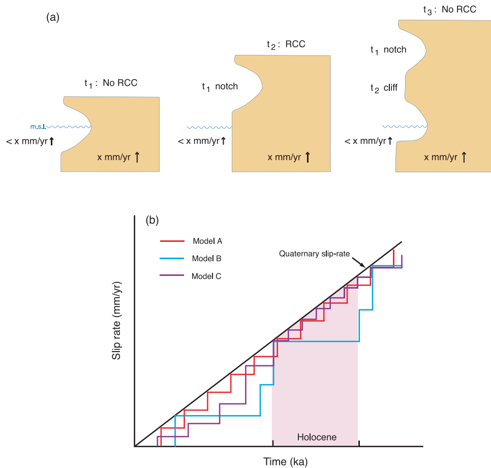
Figure 4. (a) A schematic illustration of notch formation related to climate stability. The coastline uplifts at a rate of x mm/yr while mean sea level rises but does not keep pace with coastal uplift ( < x mm/yr). At time 1 ( t_1 ), there is no RCC, providing stable conditions for organisms to carve a notch in the sea cliff. By time 2 ( t_2 ) the notch formed at t_1 has been uplifted out of the water and climate is now unstable (RCC). This means that organisms are unable to carve a new notch, so the steep sea-cliff remains. At time 3 ( t_3 ), both the t_1 notch and t_2 sea-cliff are uplifted out of the water and a new period of climatic stability allow organisms to create a new notch at sea level. (b) Three hypothetical slip-rate models for the South Alkyonides Fault.
