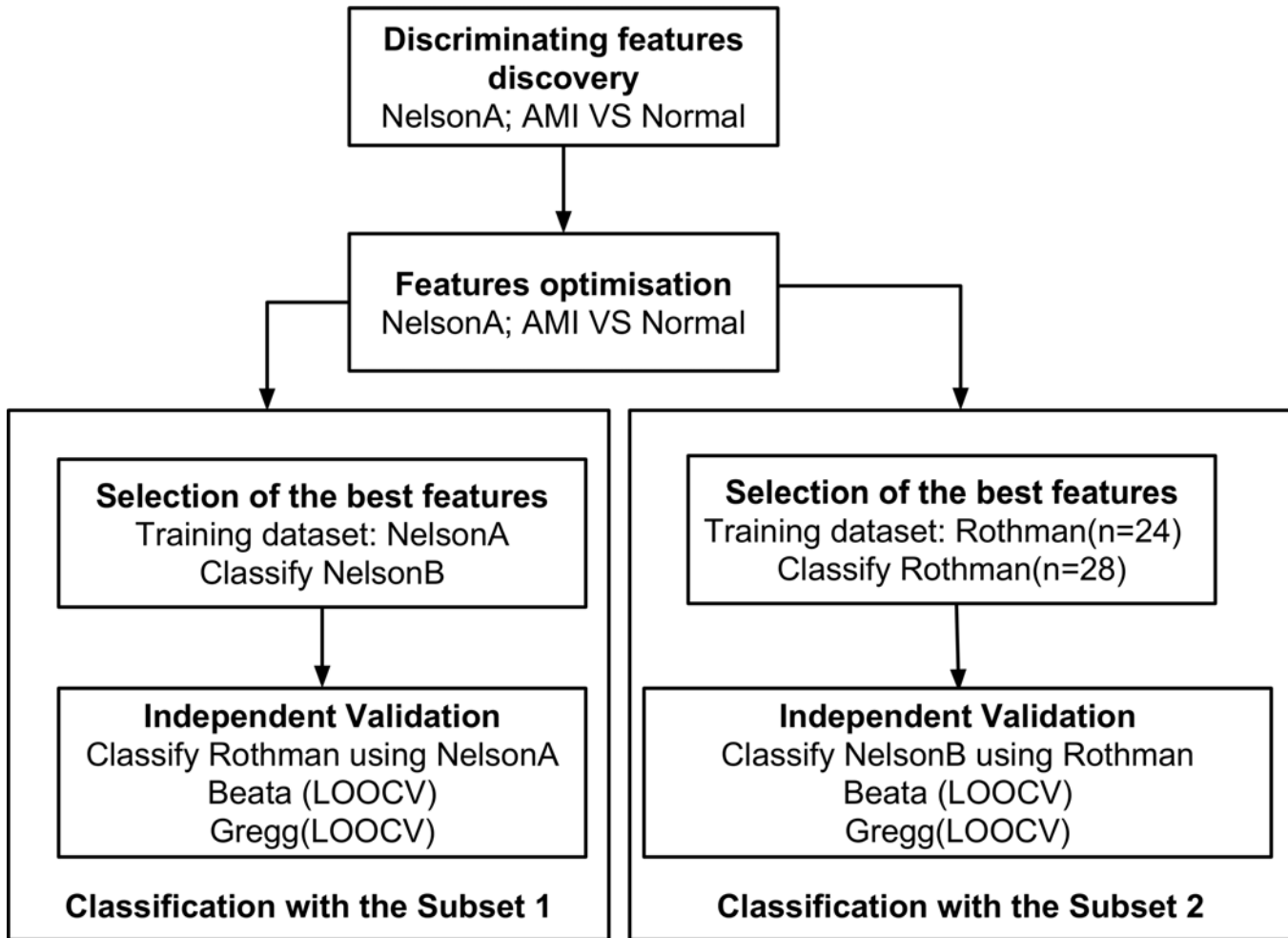
Fig 1. A flow chart to describe the classification process.
