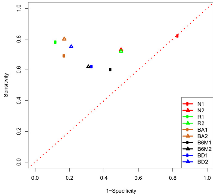
Fig 3. The ROC graph is plotted to show the performance of the binary classifiers.
