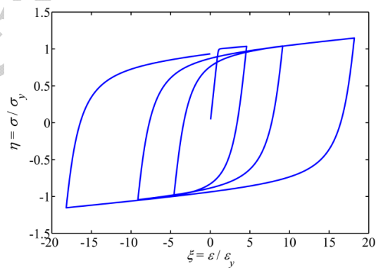
Fig. 5 Cyclic response of Steel02 material model
