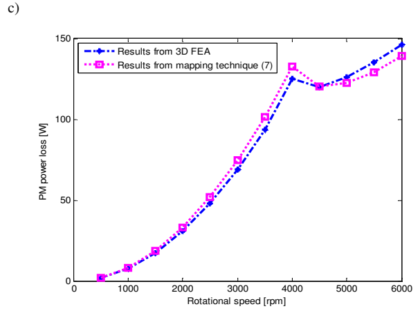
Fig. 15. Estimated magnet loss over the torque-speed envelope a) axial 7 segments PM array, b) axial 19 segments PM array, c) circumferential 4 and axial 7 segments PM array
