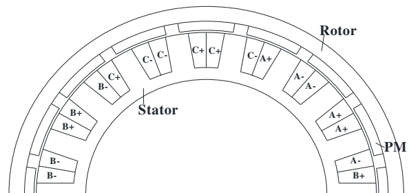
Fig. 1. Cross-section of the analysed PM motor design -2D FE model representation
