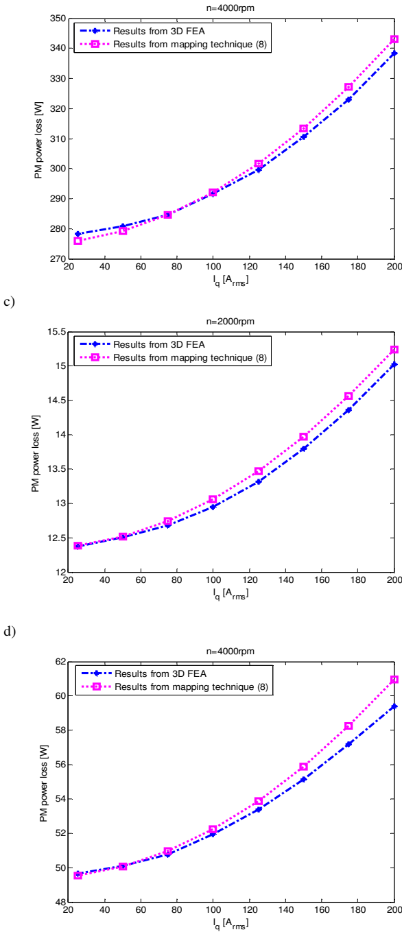
Fig. 11. PM power loss versus excitation current I_{ph} = I_q and rotational speed for maximum torque per Ampere operation, a), b) 7 segment PM array n = 2000\text{rpm} , n = 4000\text{rpm} , c), d) 19 segment PM array, n = 2000\text{rpm} , n = 4000\text{rpm}
