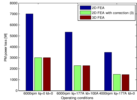
Fig. 8. PM power loss predictions at a number of operating points employing various FE based PM loss derivation techniques
