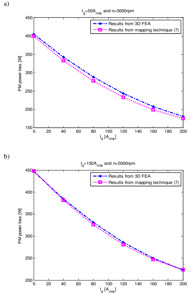
Fig. 12. PM power loss vs. I_d current, a) I_q = 50\text{A}_{\text{rms}} , n = 5000\text{rpm} , b) I_q = 150\text{A}_{\text{rms}} , n = 5000\text{rpm} - 7 segment PM array
