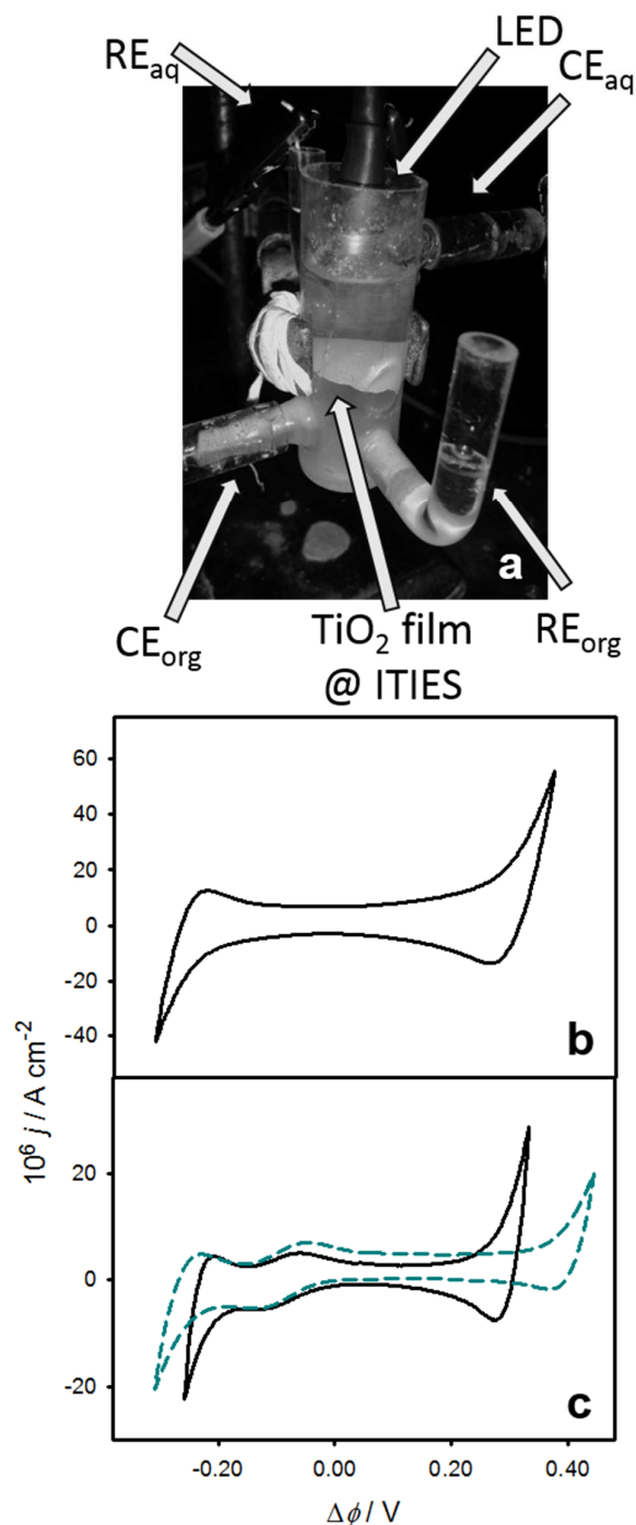
Figure 1. Three-compartment electrochemical cell featuring reference (RE) and counter electrodes (CE) in the aqueous (top) and organic electrolytes (bottom), as well as a layer of coalesced 25 nm TiO 2 particles (a). The LED used for photoexcitation is located at the top of the cell. Cyclic voltammogram of Cell 1 in the presence of the coalesced TiO 2 particle (25 nm) layer at the water/DCE interface at 0.05 V s -1 (b). Cyclic voltammograms of cells 1 (coalesced TiO 2 nanoparticle layer) and 2 (5 nm TiO 2 aqueous colloidal solution) at 0.05 V s -1 (c). The composition of the electrochemical cells can be found in the ESI. Both cells show the characteristic ion transfer responses associated with the transfer of the 1,1'-dimethylferrocenyl cation (DMFc + ) accumulated after prolonged illumination. The shorter potential window in Cell 1 is due to the higher concentration of LiCl in the aqueous electrolyte, in comparison to Cell 2.
