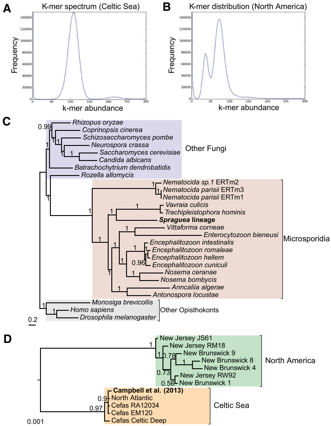
Fig. 2. Evidence for a whole-genome duplication at the base of the North American clade. (A) The unimodal k-mer distribution for a representative Celtic Sea genome, that of the “Celtic Deep” isolate. (B) The k-mer distribution for a representative North American genome, the “New Brunswick 4” isolate. This distribution is bimodal, with peaks at 37\times and 74\times , suggesting the presence of both homozygous and heterozygous positions in North American genomes, but only homozygous positions in the Celtic Sea population. (C) A Bayesian phylogeny of the Spraguea lineage in the context of its microsporidian relatives and other opisthokont outgroups. Within- Spraguea relationships are collapsed due to the relatively short branch lengths in this region of the tree. (D) Relationships among Spraguea isolates, rooted using the tree depicted in (C). The earliest divergence splits the North American and Celtic Sea isolates with maximal posterior support (PP = 1), placing the ploidy increase at the base of the North American clade. These trees were inferred under the CAT + GTR model (Lartillot and Philippe 2004) in PhyloBayes-MPI 1.5a (Lartillot et al. 2013) using a concatenation of 23 single-copy orthologous protein-coding genes that share a congruent phylogenetic signal as determined by a hierarchical likelihood ratio test (Leigh et al. 2008).
