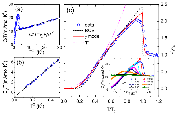
FIG. 3: (Color online) (a) Specific heat C/T against T^2 for \text{LaNiGa}_2 . The solid line shows a linear fit above T_c . (b) The electronic specific heat C_e/T against T^2 at low temperatures. The solid line shows a linear fit which extrapolates to negative C_e/T . (c) Temperature dependence of C_e/T , normalized to the normal state value. The solid line shows the \gamma model fit, while the dashed and dotted lines show the behavior of a weakly coupled, isotropic BCS superconductor and a T^2 dependence respectively. The inset shows C_e/T(T) in various applied magnetic fields
