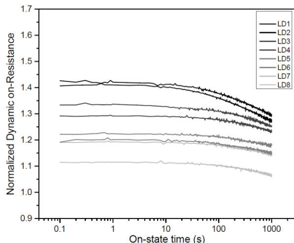
(b) Large devices at RT
