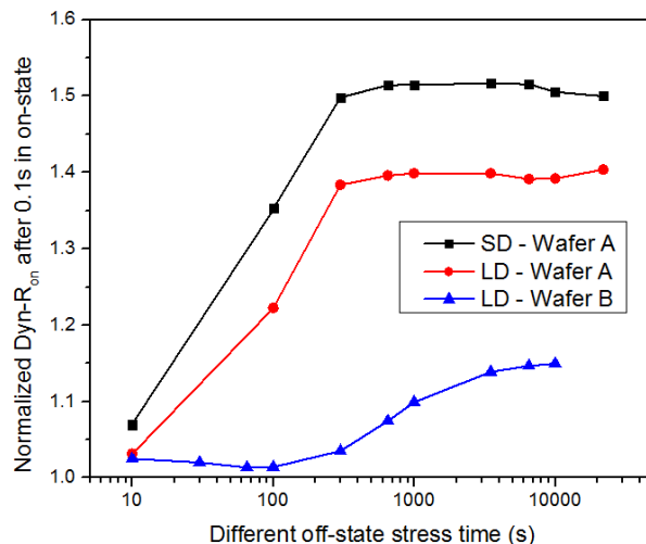
Fig. 4. Normalized Dyn-Ron at 40°C, 0.1s after switching to on-state for small (SD) and large (LD) devices from wafers A and B.
