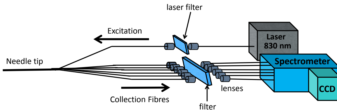
Fig. 2. Schematic diagram depicting the Raman needle probe instrumental setup. Excitation at 830 nm was provided by a CW IPS laser passing via fibre optic cable through a short pass filter ('laser filter'), and into the central fibre of the needle tip. The six collection fibres returning from the needle tip were directed through a long pass filter ('filter') and were delivered to the spectrometer in a vertical column across the entry port. Spectra were acquired with a deep depletion CCD camera.
