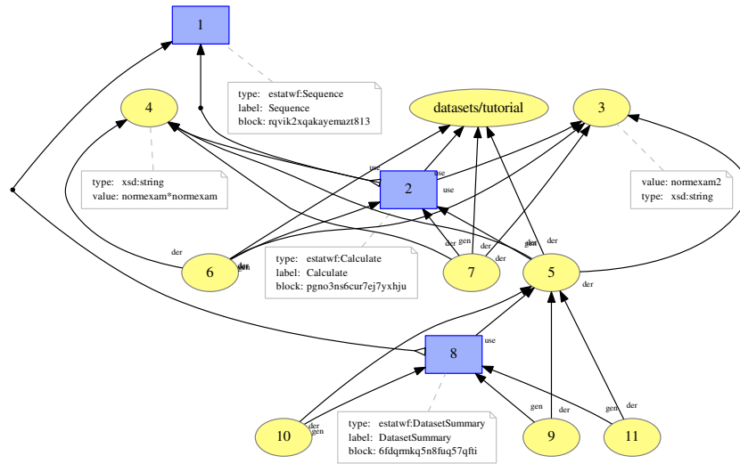
Fig. 6. Provenance graph derived from expansions of template of Fig. 5 and INPWR records of Fig. 3.
