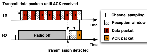
Fig. 1: A representative scheme from LPL MAC protocols. Nodes sample the medium periodically to detect a transmission. If a carrier is detected, the receiver keeps its radio ON to receive the associated data packet(s).
