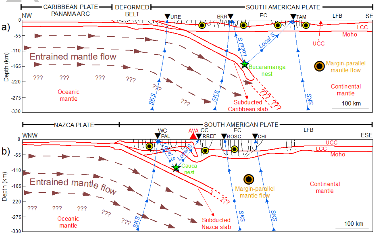
Figure 9. Regional sections showing the general interpretation of the S -wave splitting results north and south of the Caldas Tear. a) and b) correspond to the profiles AA' and BB' respectively in Figure 4. The ongoing underthrusting of the coupled Panama arc/Caribbean plate to the north of Caldas Tear is responsible for a strong SKS splitting signal beneath the descending slab by means of entrained mantle flow parallel to the direction of subduction. Similarly, south of Caldas Tear, the SKS anisotropy is reflecting a mechanical coupling between the descending Nazca slab and the mantle beneath it, but in this case, the splitting signal is weaker due to the steeper subduction angle. Further inland, there is an asthenospheric flow that is parallel to Pacific and Caribbean continental margins (orange/black circle) and is probably related to the northeastward motion of the North Andes block. Local S splitting appears to be strongly controlled by crustal-scale fault zones (bold black lines), therefore the anisotropy signal would be restricted to the continental crust (yellow/black circle). Finally, the mantle wedge is interpreted as apparently isotropic. Inverted black triangles are stations, and the red triangle indicates the location of the active volcanic arc (AVA). Blue arrows show the trajectories of SKS and local S phases. UCC: Upper Continental Crust; LCC: Lower Continental Crust; LFB: Llanos Foreland Basin; WC: Western Cordillera; CC: Central Cordillera; EC: Eastern Cordillera.
