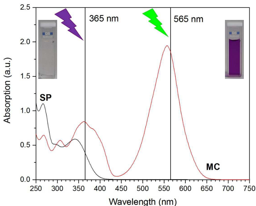
Figure 1: top: Switching states of spiropyrans. The closed spiropyran form ( SP ) undergoes a ring opening upon irradiation with UV light (365 nm, purple flash) to the open merocyanine form ( MC ). Irradiation with visible light (565 nm, green flash) induces a ring closure and drives the equilibrium towards the SP side. Bottom: Absorption spectra and photographs of the two states. The absorption spectrum of the SP is plotted in black, the spectrum of the MC in red. Flashes and vertical lines represent the wavelengths used for switching. Whereas the colorless SP form does not absorb at wavelengths higher than 400 nm, the solution of MC shows a dark purple color which results from a broad absorption with a maximum wavelength of approx. 550 nm. The solution in acetonitrile had a concentration of 65 \mu\text{mol/L} and irradiation times of 30 sec were used.
