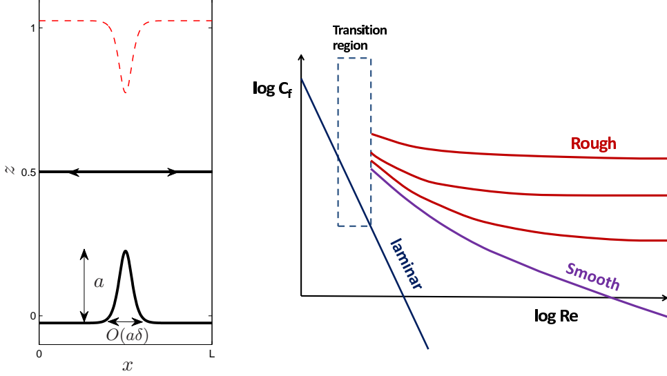
FIGURE 2. Left: the 2D ridge tidal problem with the ocean represented by the region z \leq \frac{1}{2} . Right: a cartoon of the Moody diagram for pipe flow (Moody 1944): C_f := \varepsilon/(U^3/h) , laminar flow has C_f \sim 1/Re , turbulent smooth pipe data suggests C_f \sim 1/(\log Re)^2 at least to Re = O(10^8) and turbulent rough pipe data has C_f \sim O(1) as Re \rightarrow \infty . Three lines are shown for rough pipe flow with the data increasing to higher C_f as the representative height of the roughness increases.
