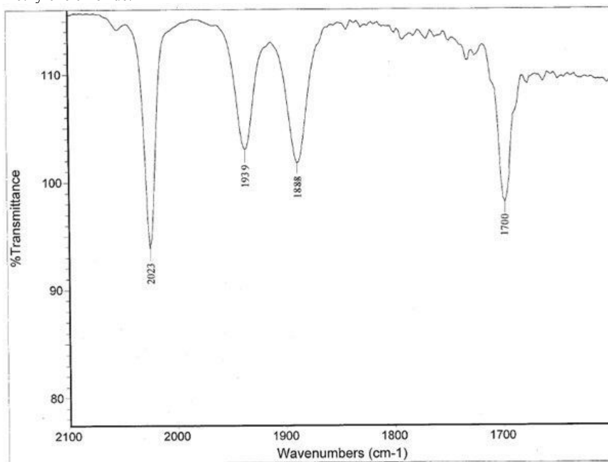
Fig. S5. IR spectrum of the reaction of [\text{Re}(\text{CO})_3(\text{dippf})\text{Br}][\text{BF}_4] with acetylferrocene in methylene chloride.
