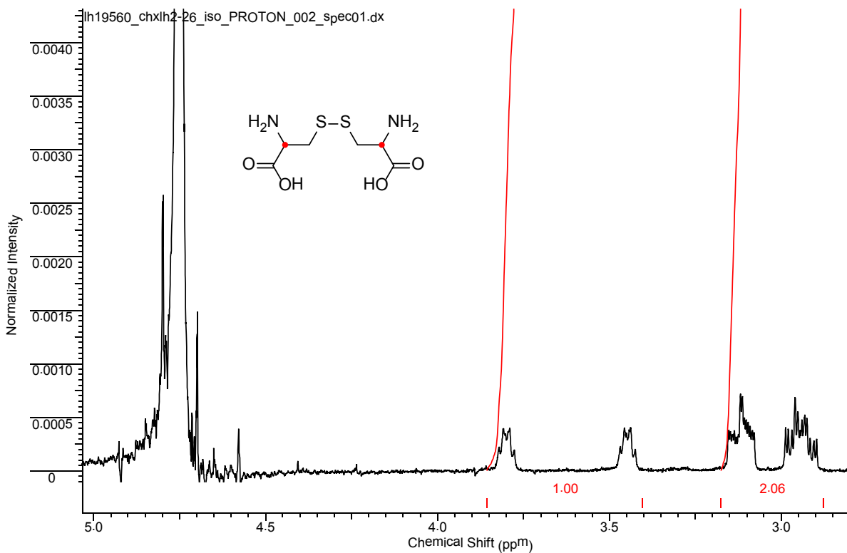
Figure S15. ^1\text{H} NMR spectrum (400MHz, \text{D}_2\text{O} ) [2-^{13}\text{C}] -cystine ( S8 ).
