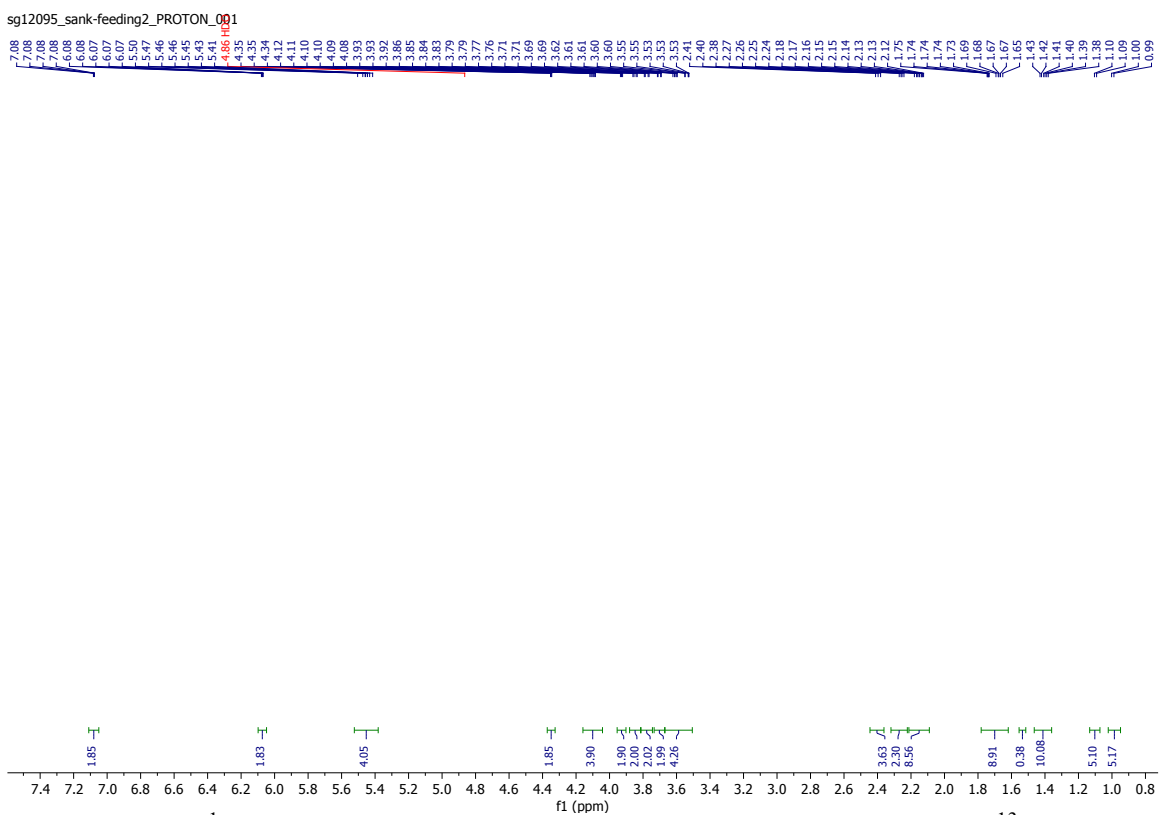
Figure S11. ^1\text{H} NMR spectrum of thiomarinol A from the feeding of [2,3-^{13}\text{C}_2] -4-hydroxybutanoic acid to Pseudoalteromonas SANK 73390 ( \text{CD}_3\text{OD} , 600MHz)
