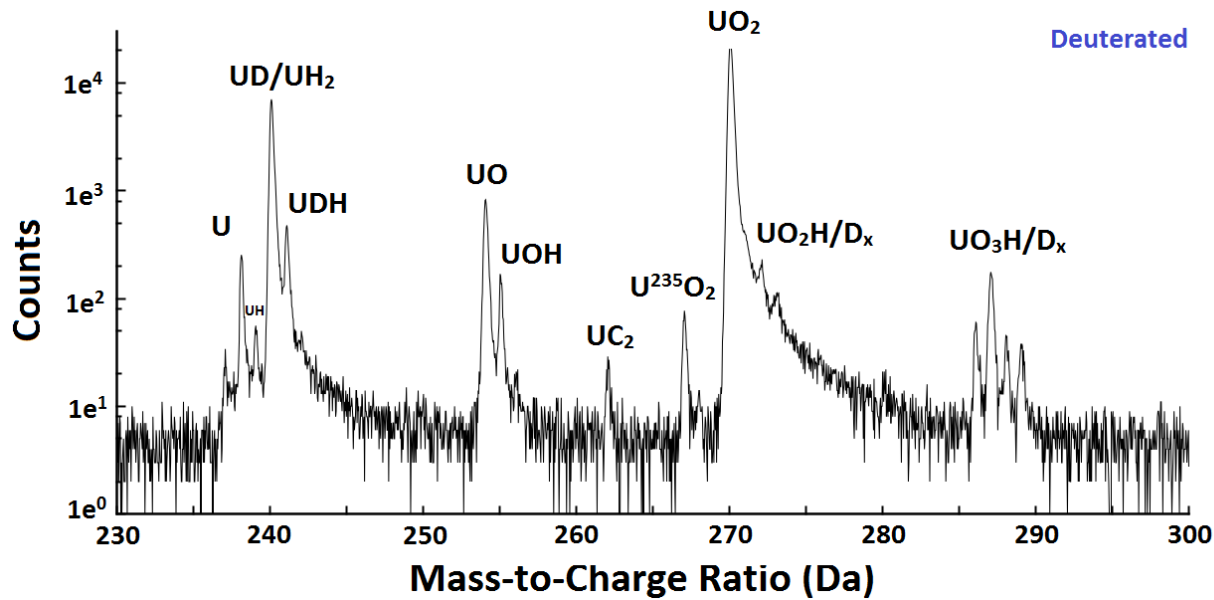
Figure S1: Mass spectrum of oxidised depleted uranium focused on the singular charged ionic states between 230 Da and 300 Da, comparing the behaviour from exposure to (a) ambient air and (b) deuterated water vapour
