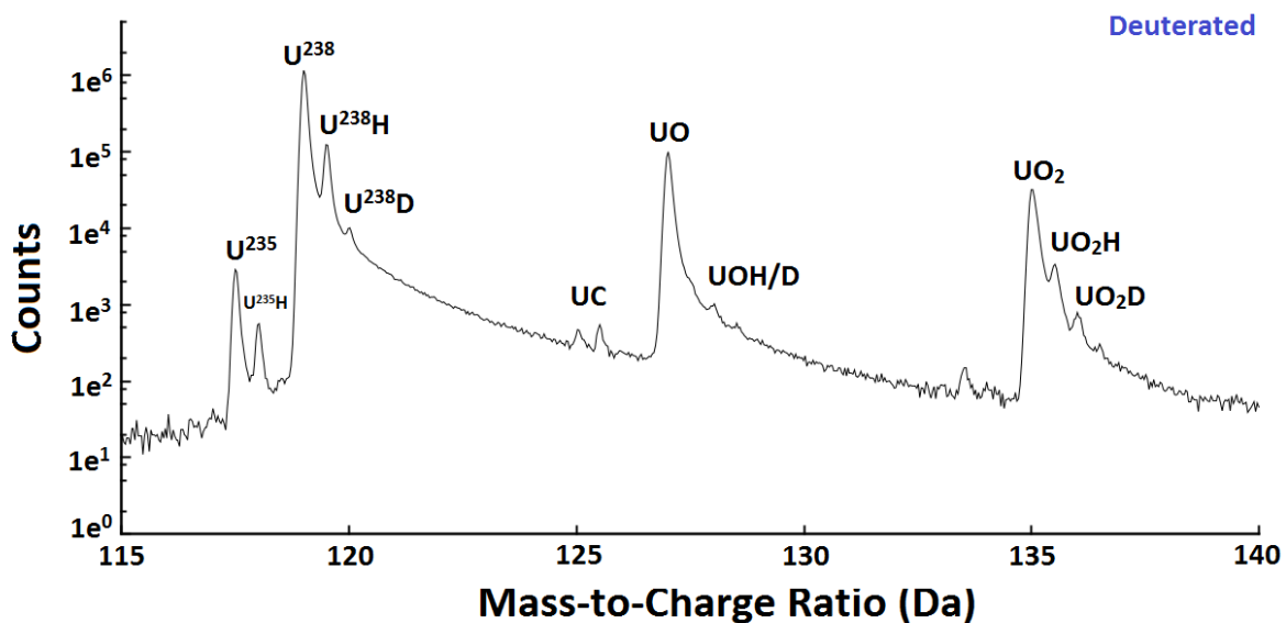
Figure S2: Mass spectrum of oxidised depleted uranium focused on the doubly charged ionic states located between 115 Da and 140 Da, comparing the behaviour from exposure to (a) ambient air and (b) deuterated water vapour
