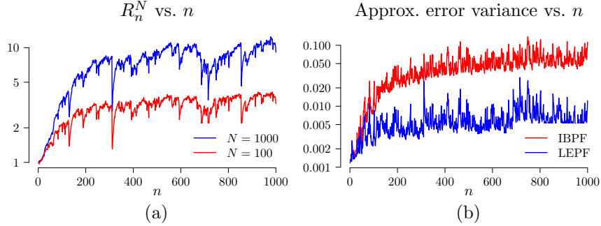
Figure 6: (a) Approximate relative variance. (b) Approximate error variance for N = 1000 .
