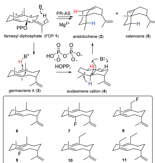
Scheme 1 Biosynthesis of (+)-aristolochene ( 2 ) and unnatural germacrene A ( 3 ) from the corresponding FDP analogues.
